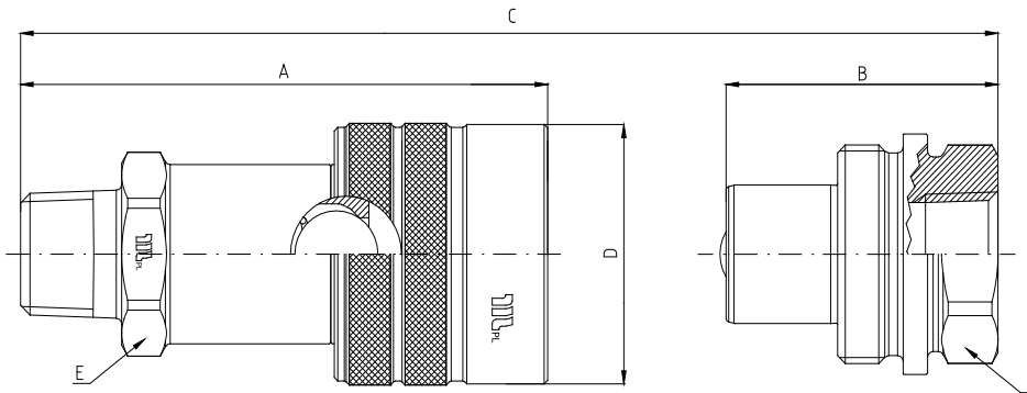
Q05611280C NPT TERMINATION ENDS TO ANSI B1.20.3
