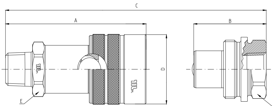
Q05510341C NPT TERMINATION ENDS TO ANSI B1.20.3
